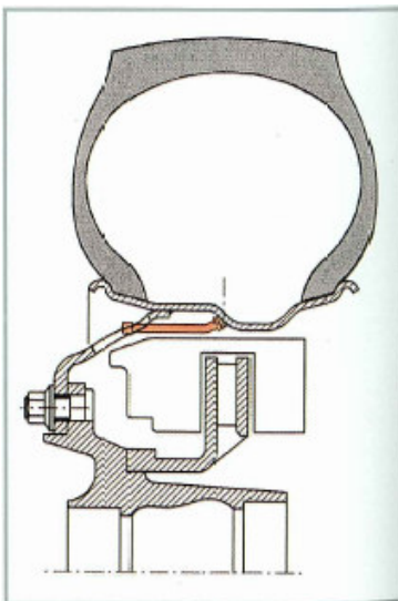
Wheel/tyre combination with 27° valve wheel
