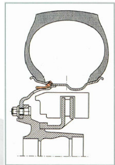
Wheel/tyre combination with 45° valve protected wheel
